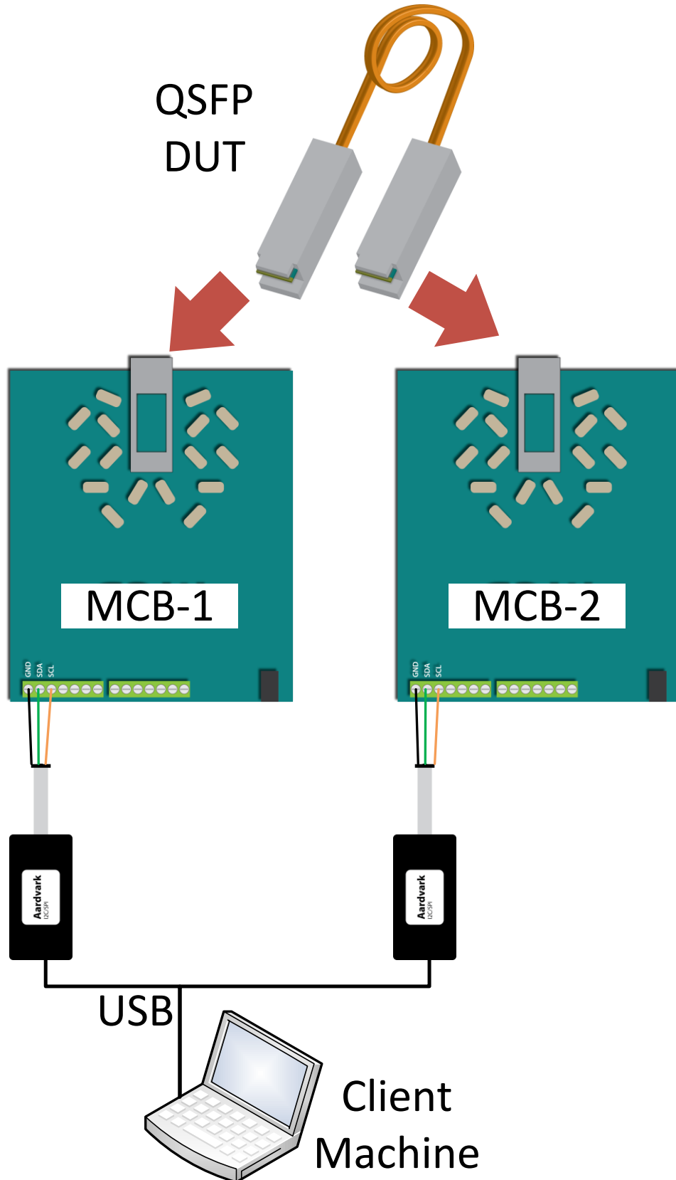
Figure 1 - ECC hardware setup
